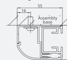
Wall mounting
